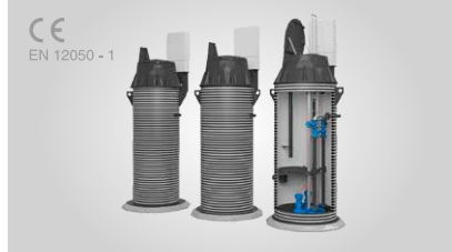
PUMPING STATIONS ID1200 – 3000 mm
