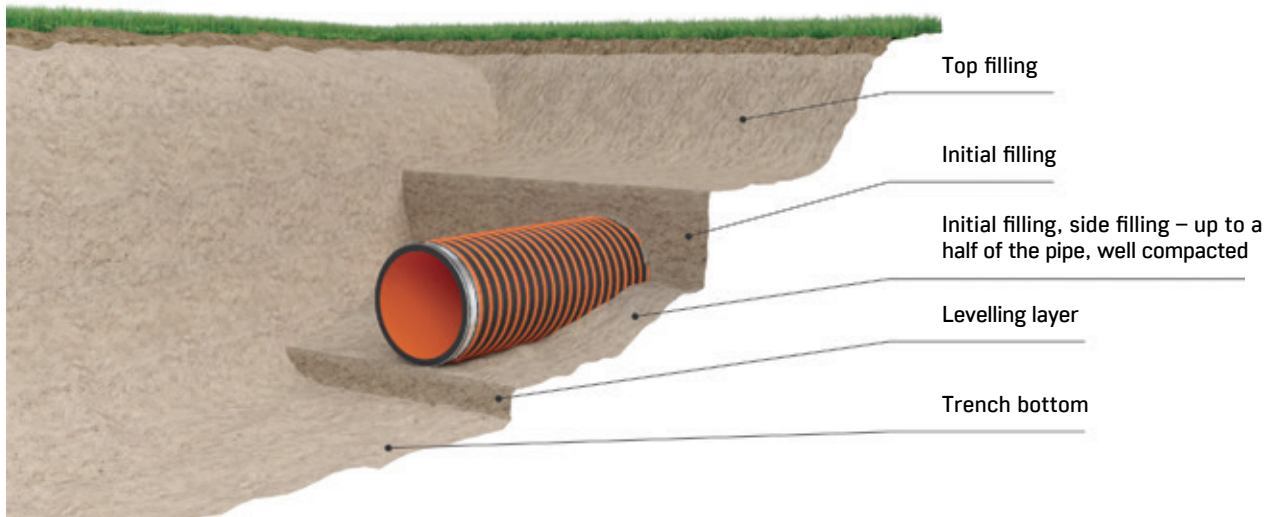
Figure 2. Trench
