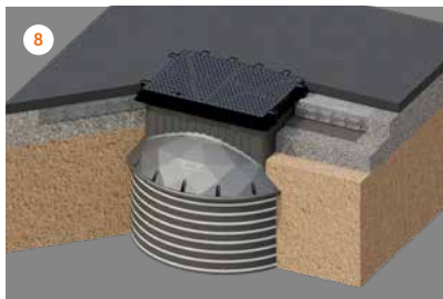
8 Install the final road pavement.
