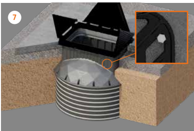
7 During installation, check the direction of the cast iron cover opening relative to the ladder. Secure the cast iron cover at the corners with wedge anchors.
